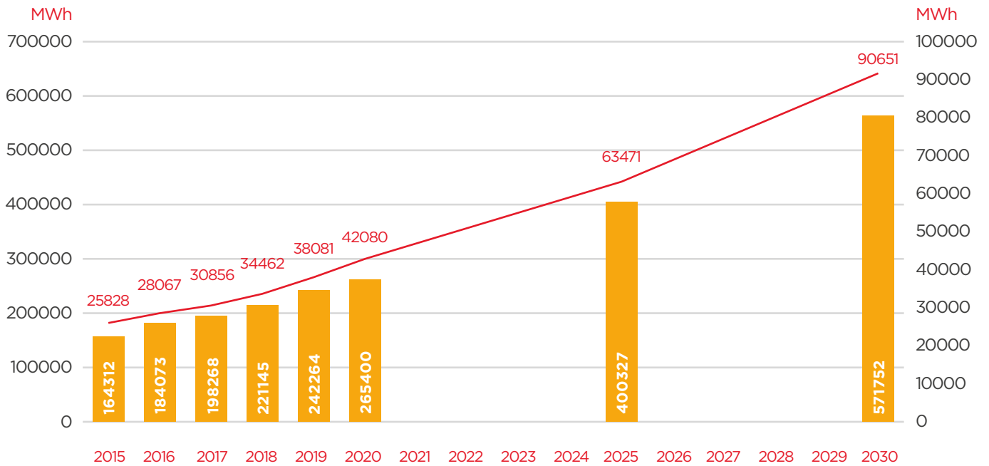
Energy Production (MWh) and Peak load (MW) from 2015 to 2030
